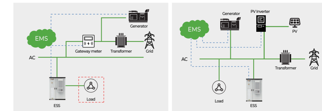
Backup Power Supply
